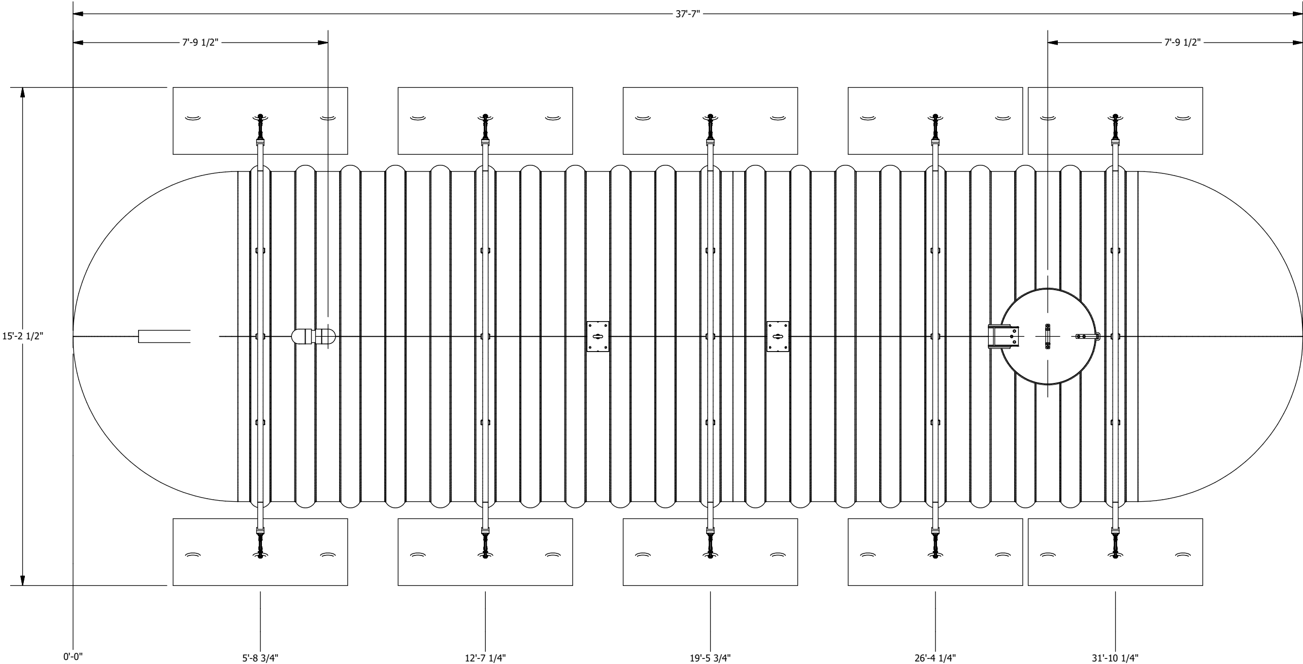
PLAN VIEW
