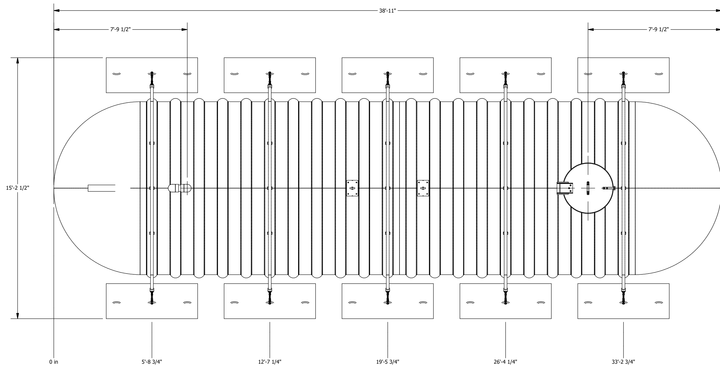
PLAN VIEW
