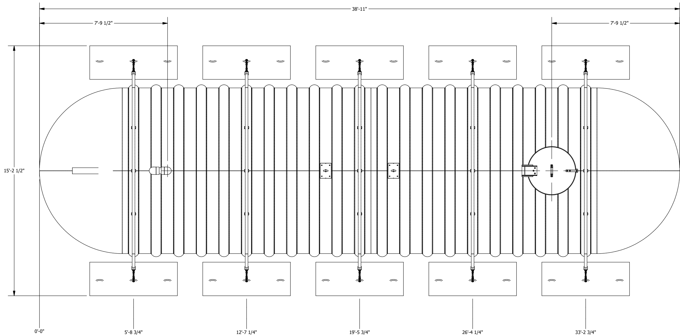
PLAN VIEW
