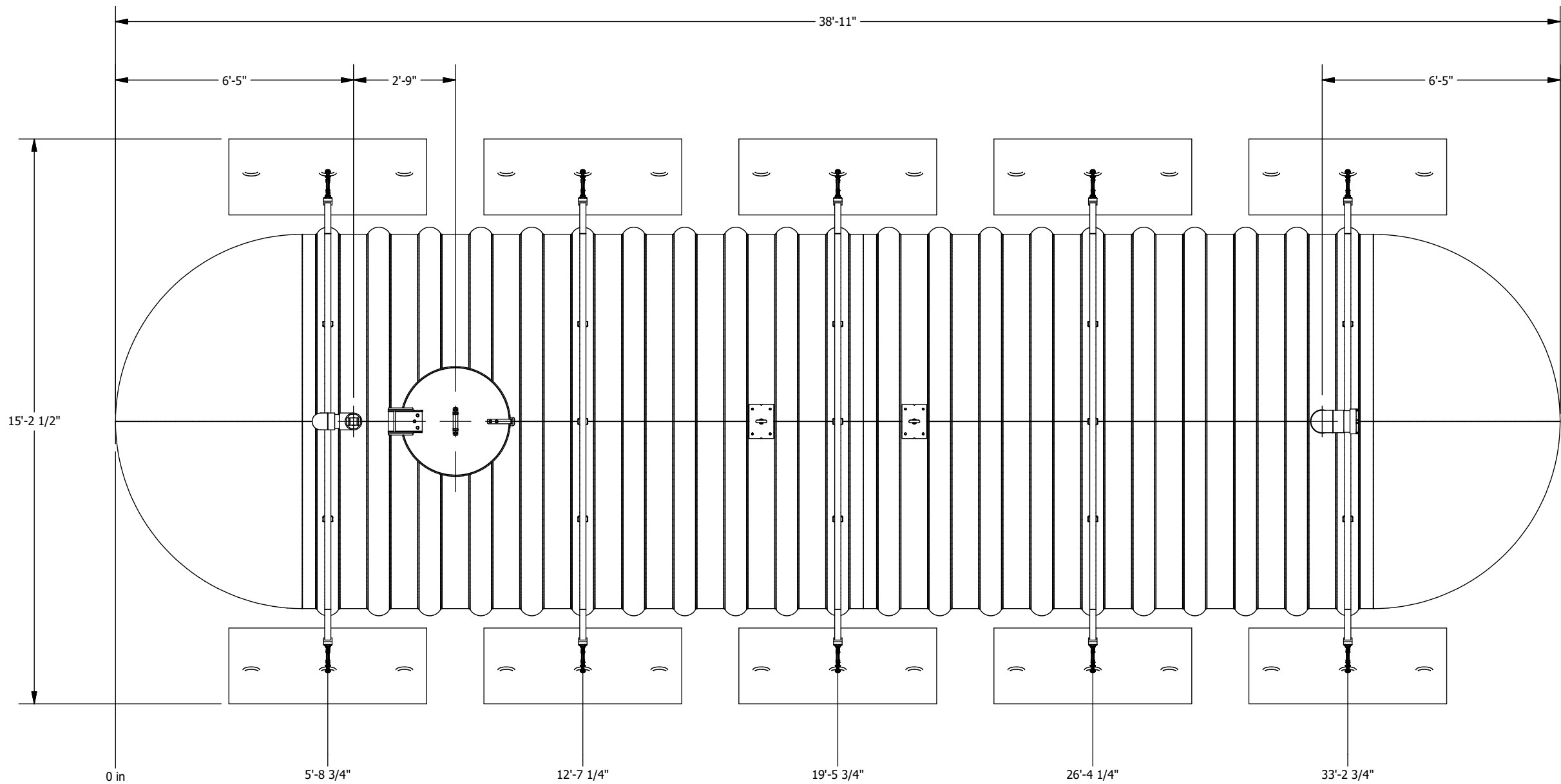
PLAN VIEW
