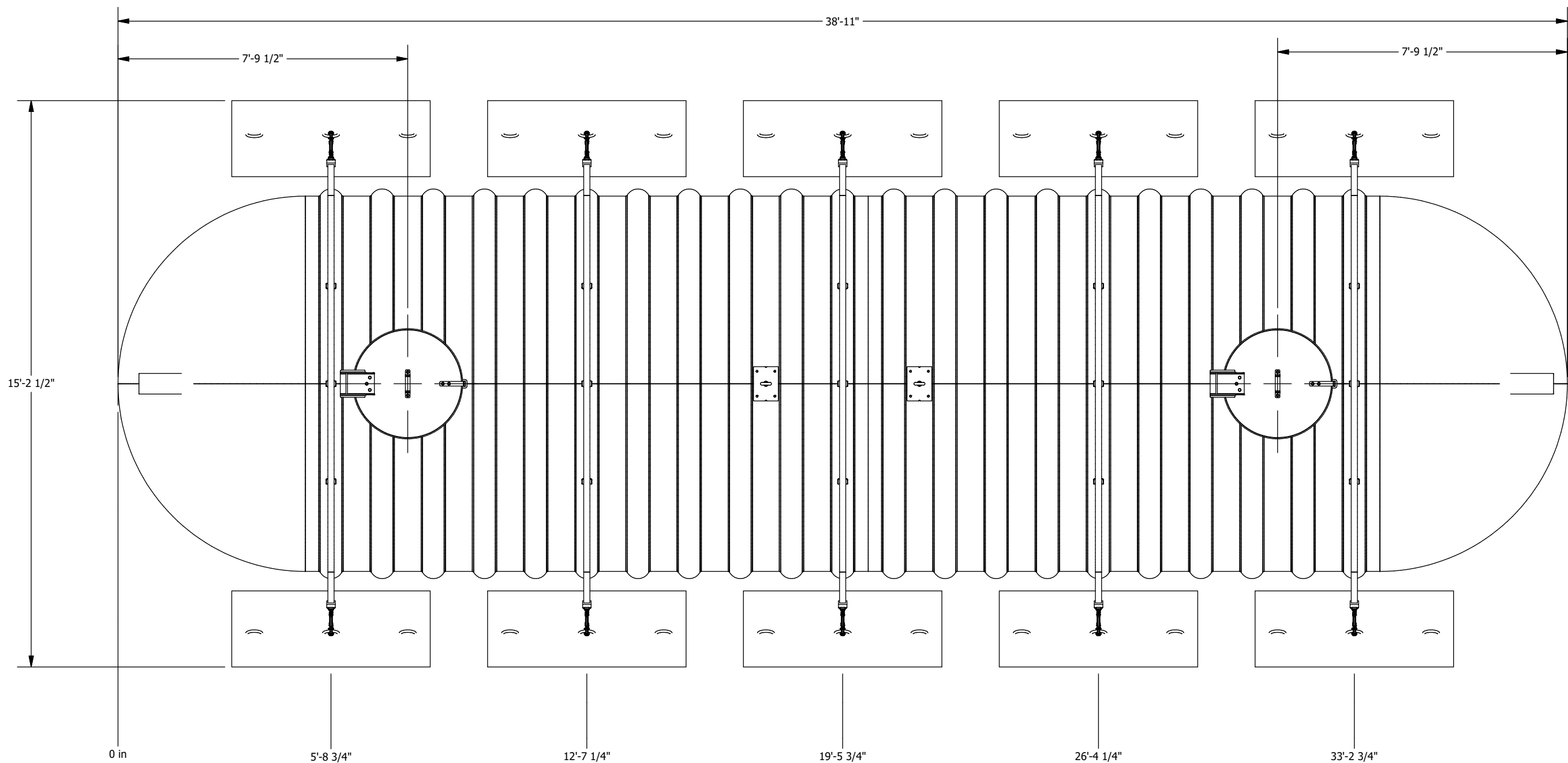
PLAN VIEW
