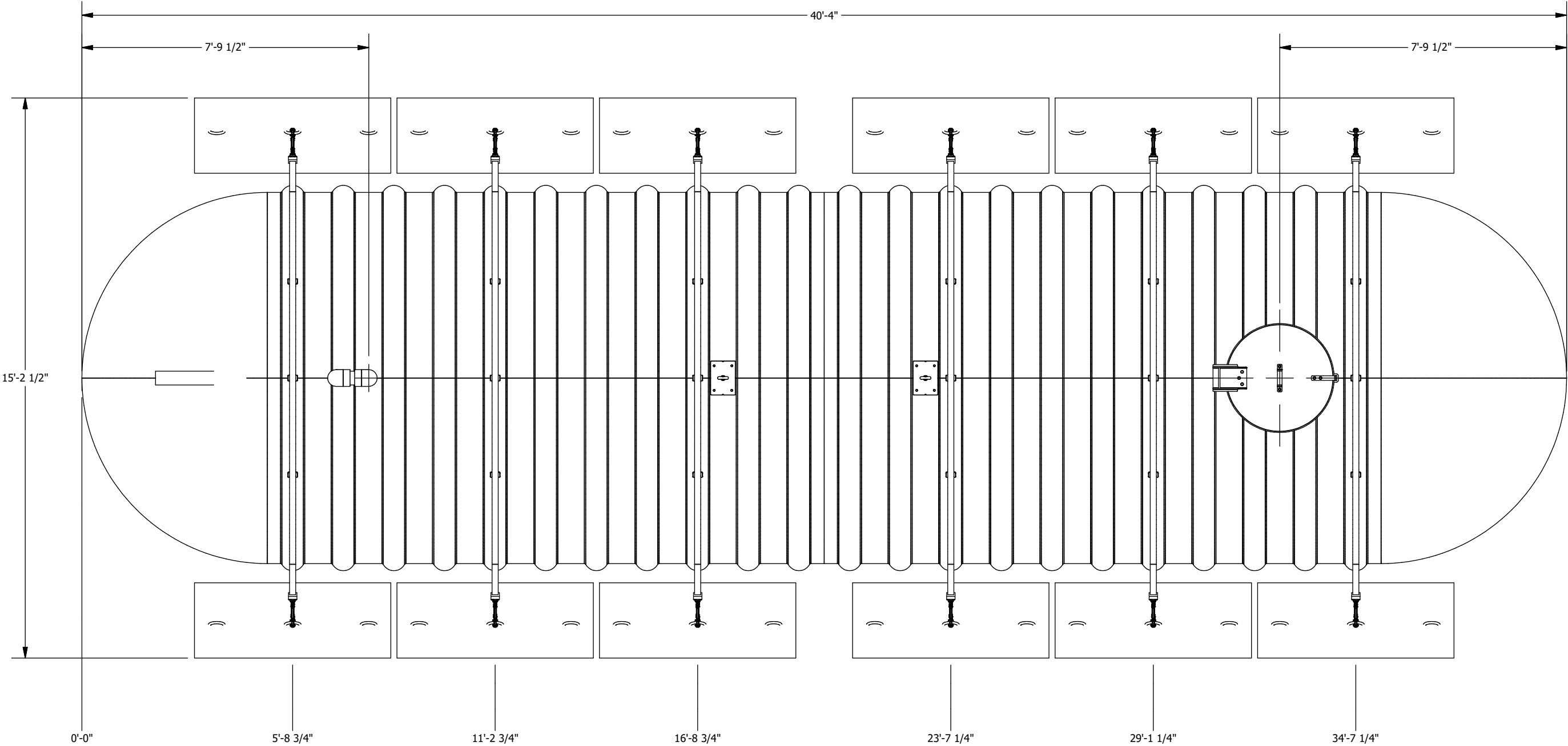
PLAN VIEW
