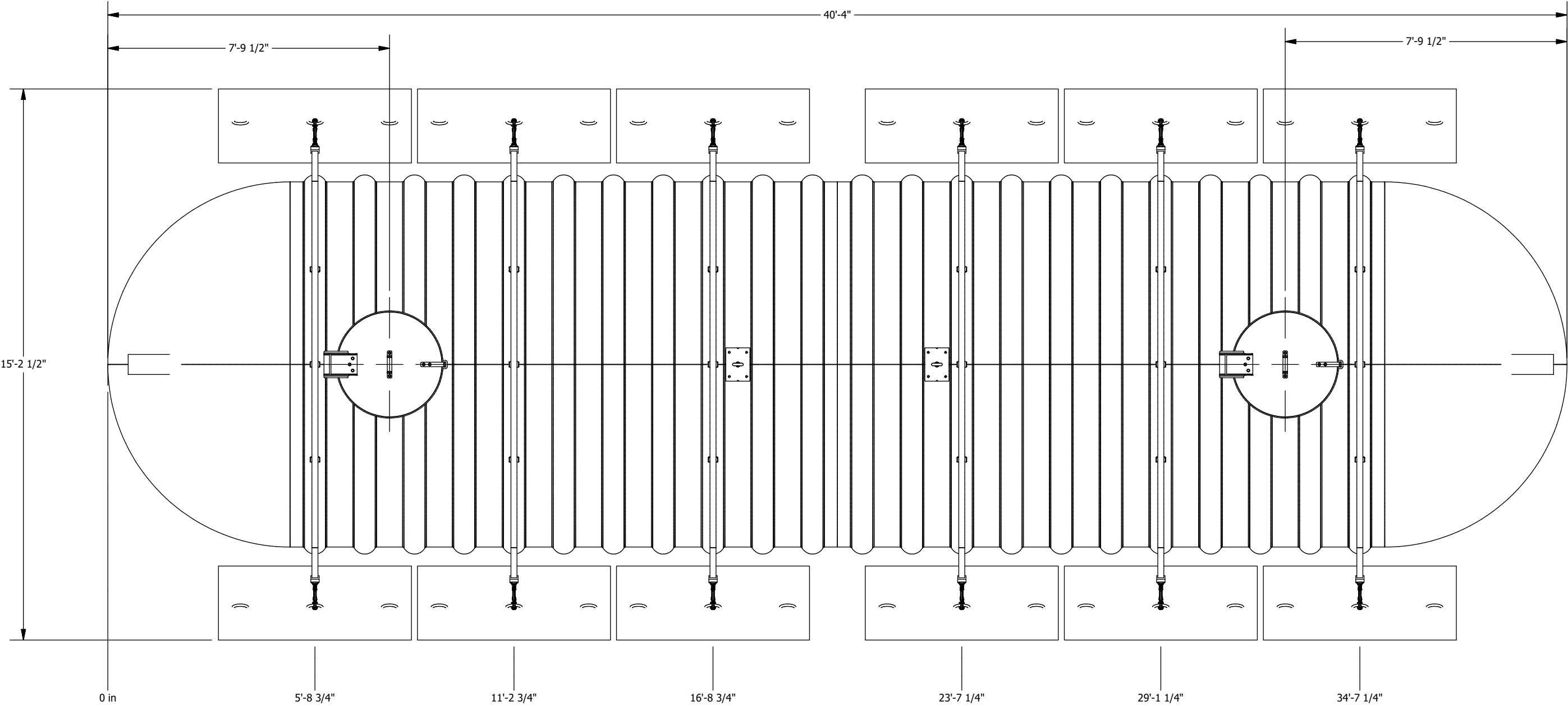
PLAN VIEW
