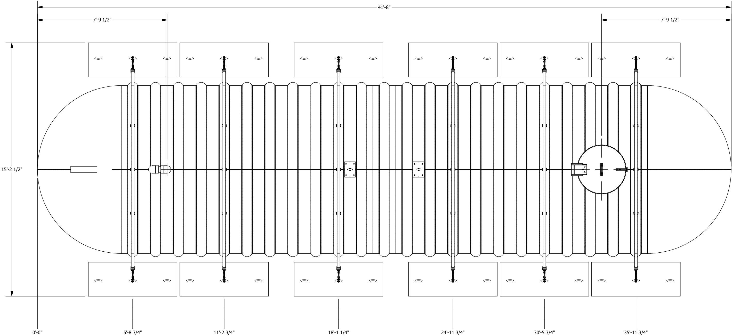
PLAN VIEW
