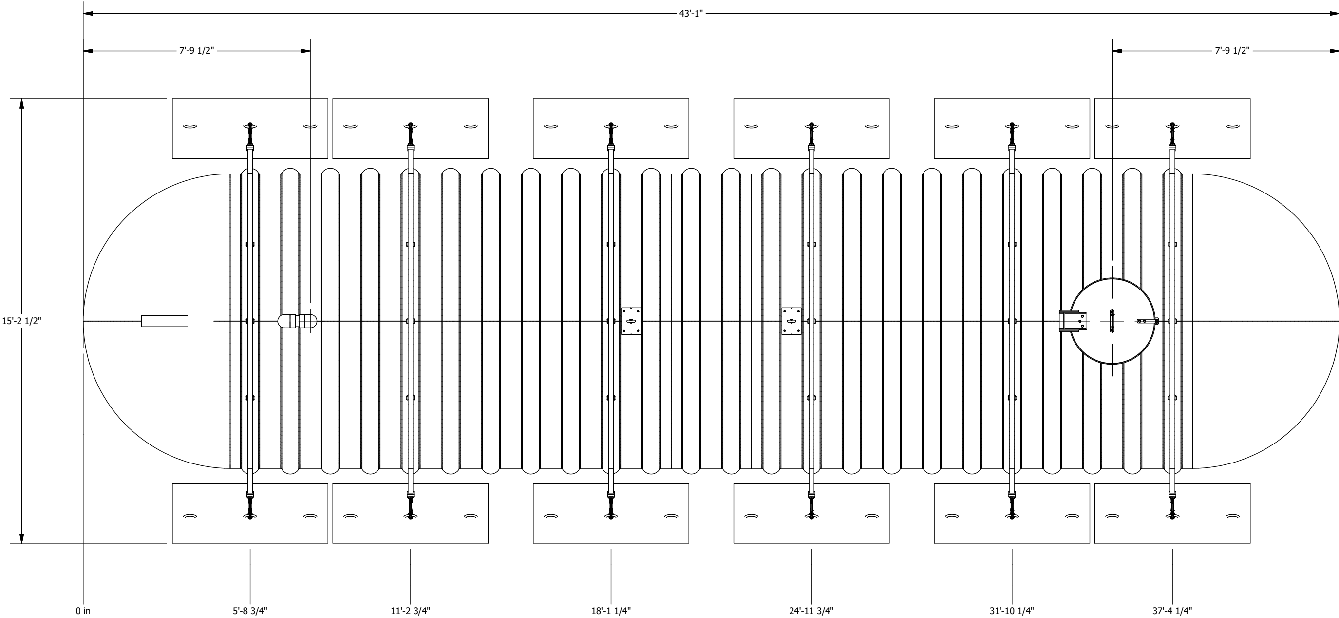
PLAN VIEW
