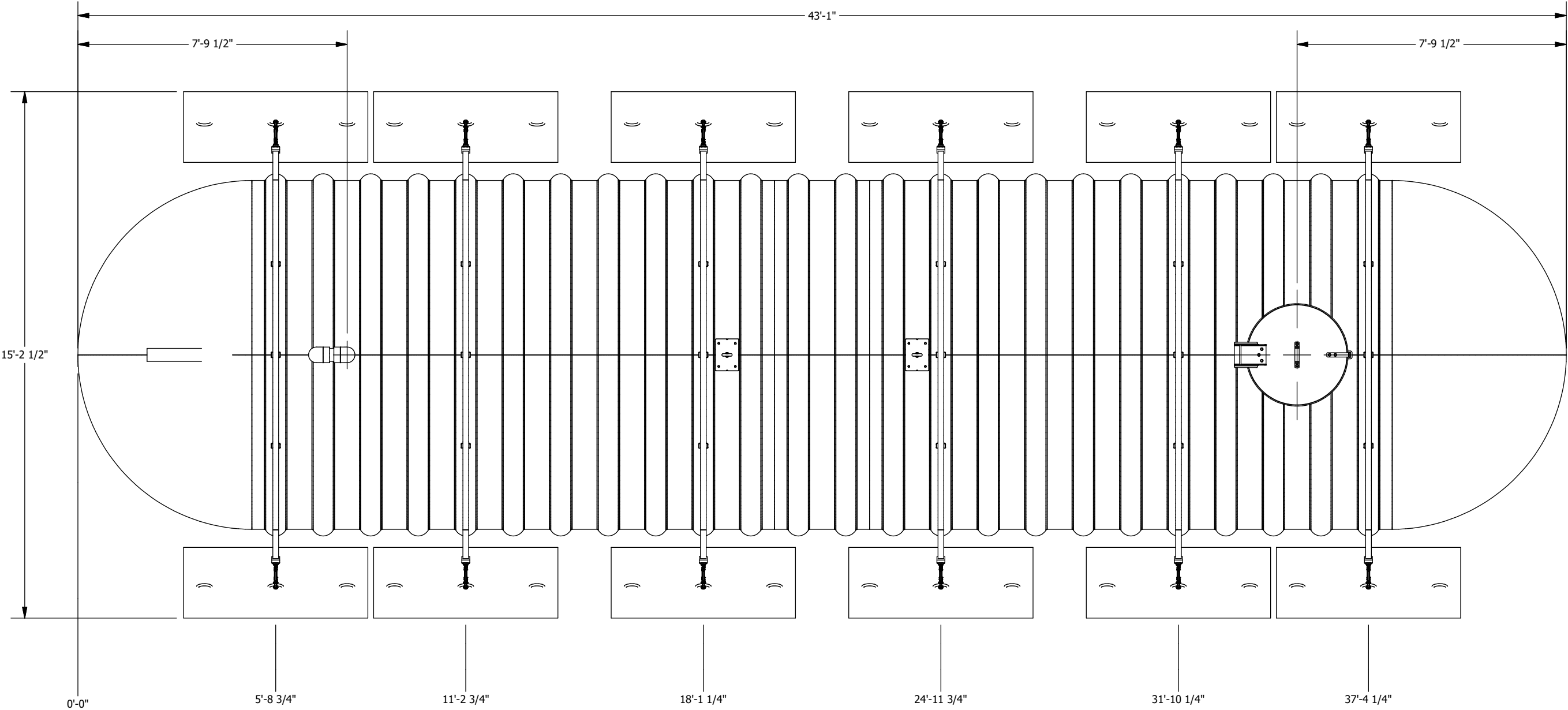
PLAN VIEW
