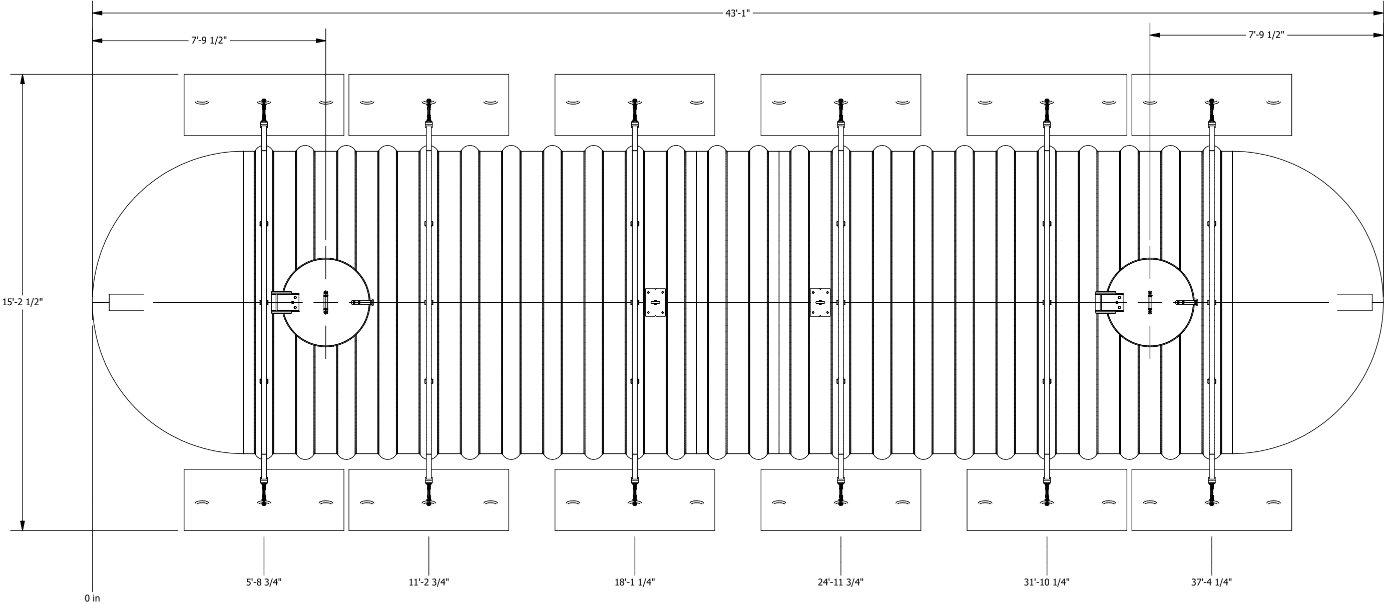
PLAN VIEW
