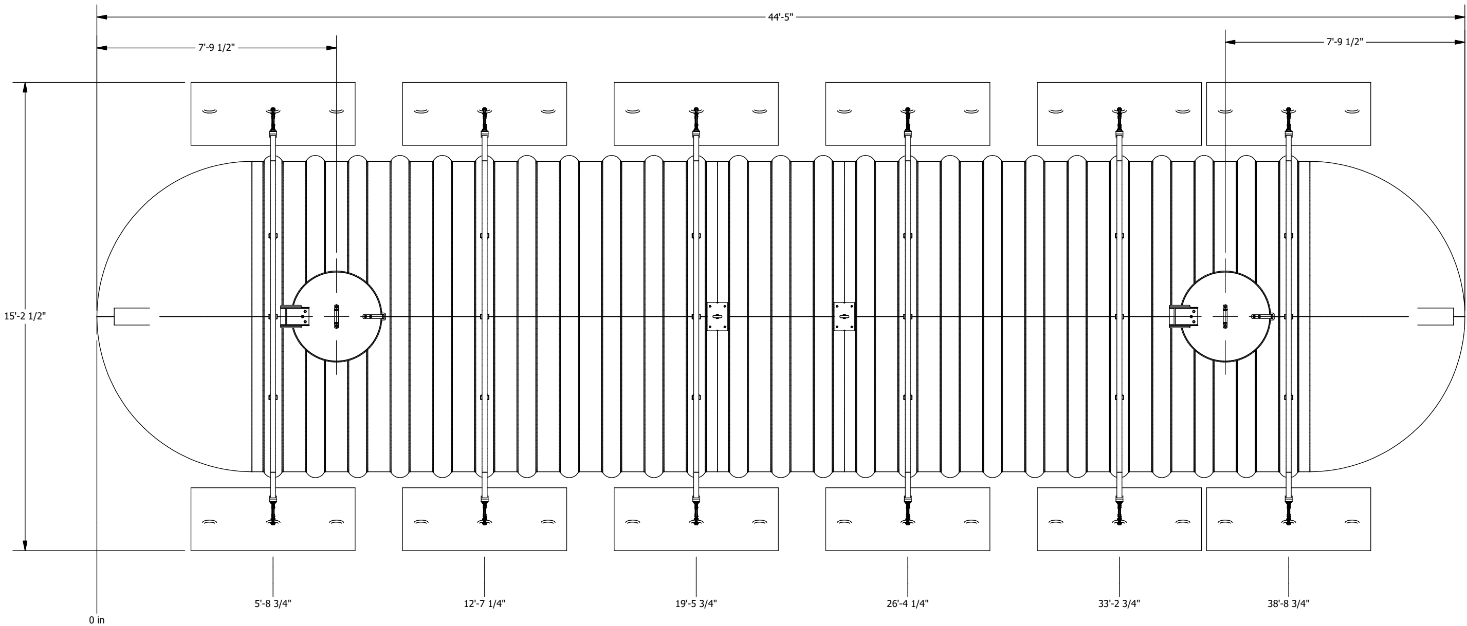
PLAN VIEW
