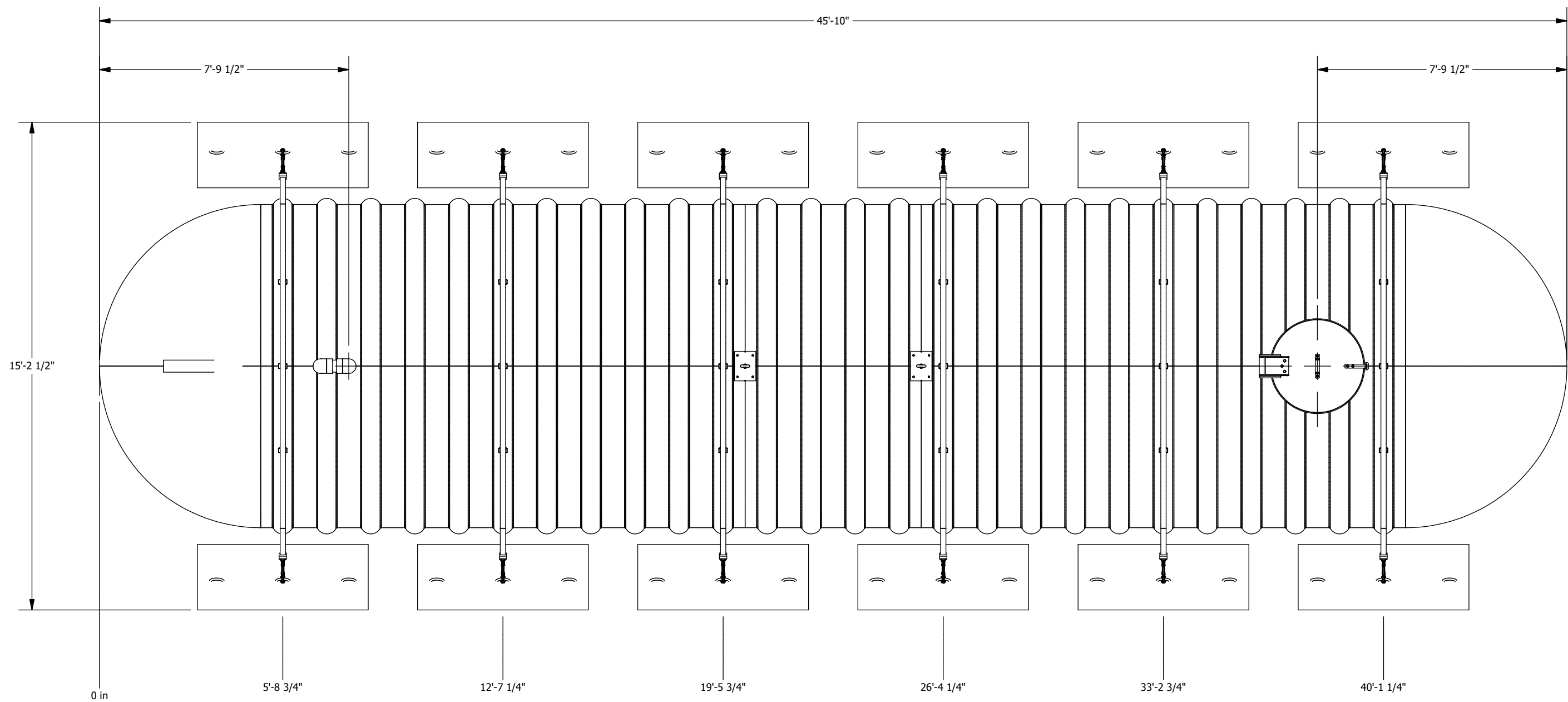
PLAN VIEW
