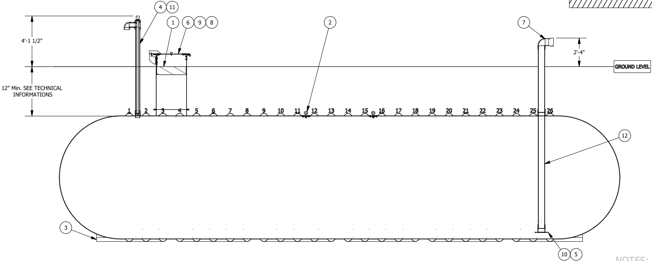
SECTION ELEVATION VIEW
