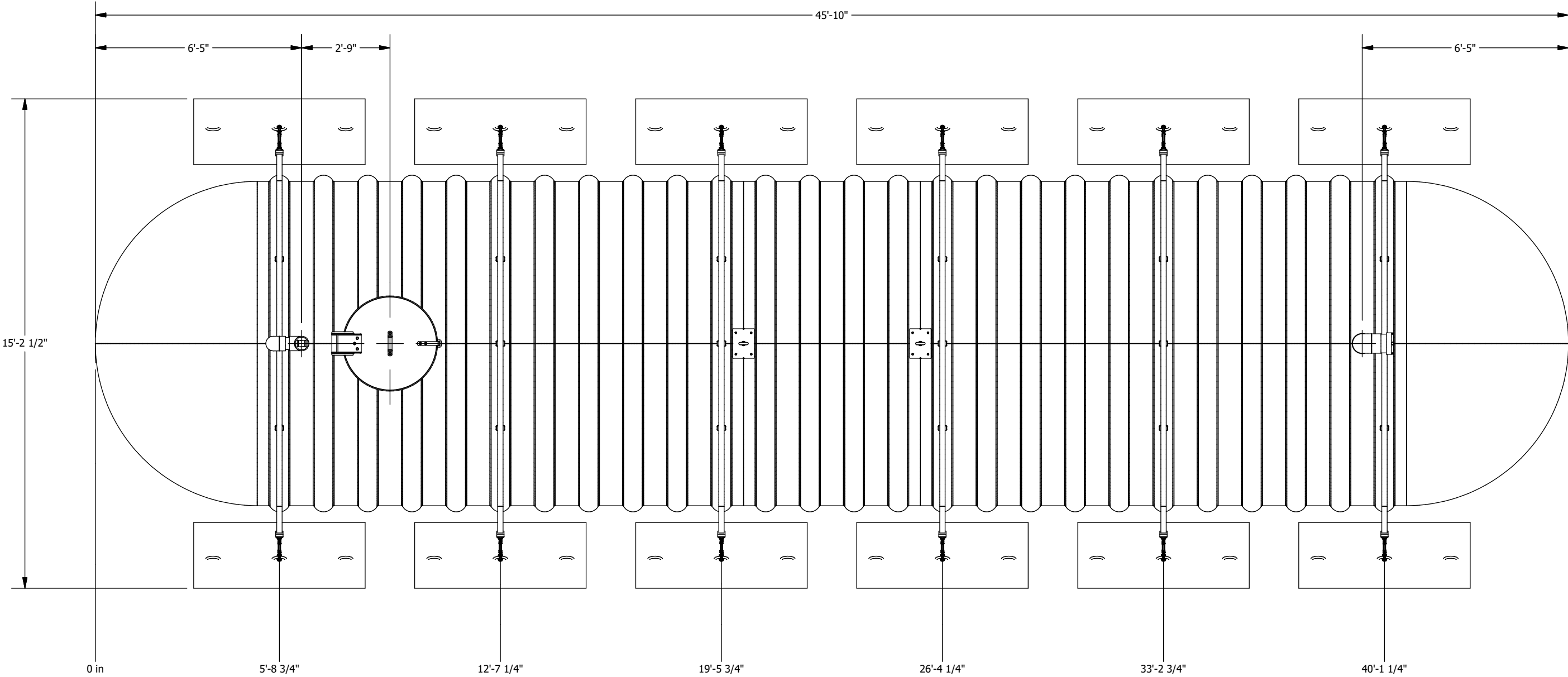
PLAN VIEW
