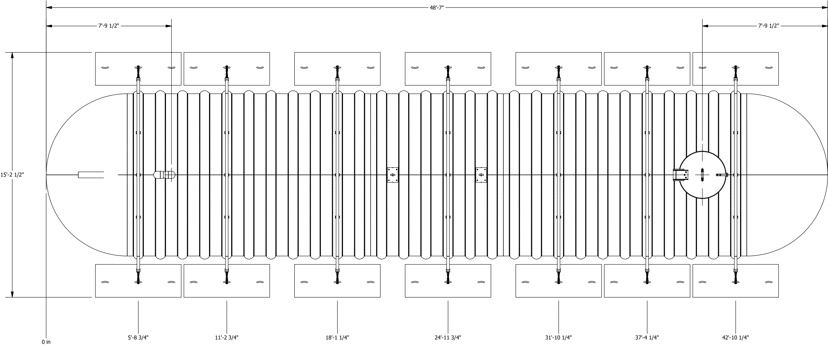
PLAN VIEW
