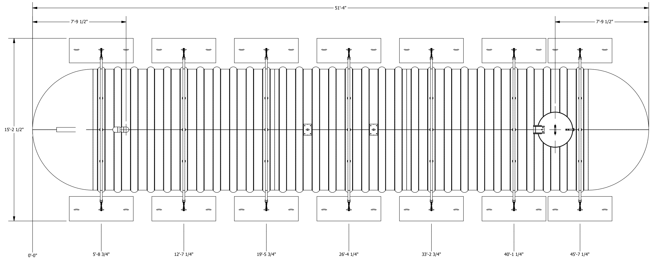
PLAN VIEW
