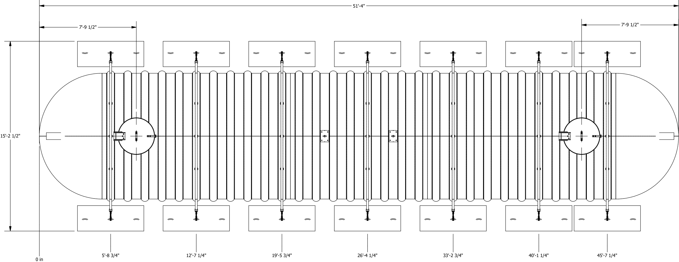
PLAN VIEW
