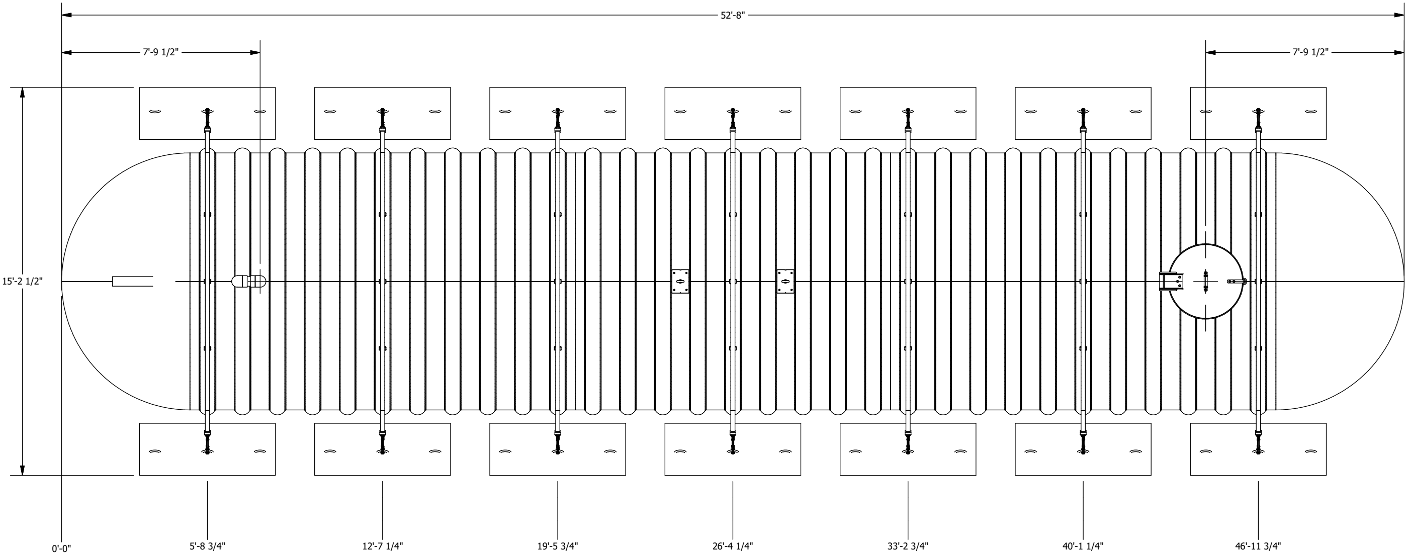
PLAN VIEW
