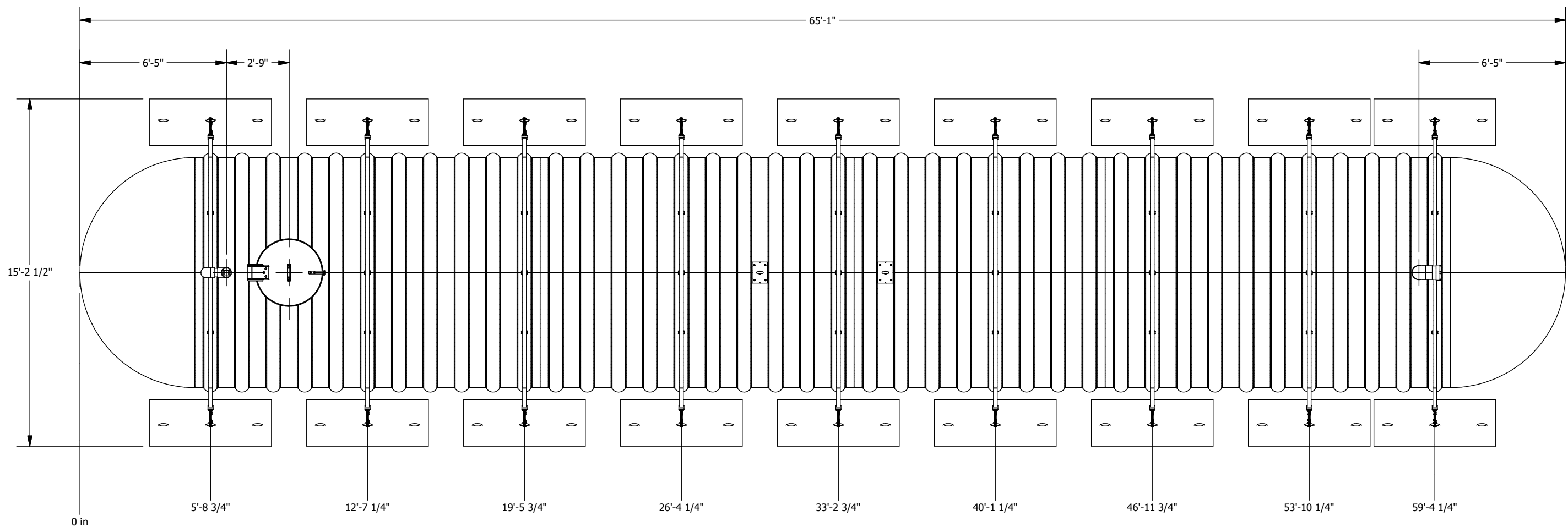
PLAN VIEW
